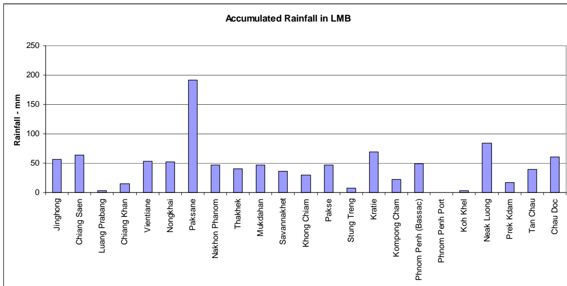
Figure 1: Accumulated Rainfall Distribution over the LMB from 04 th – 11 th September 2017
