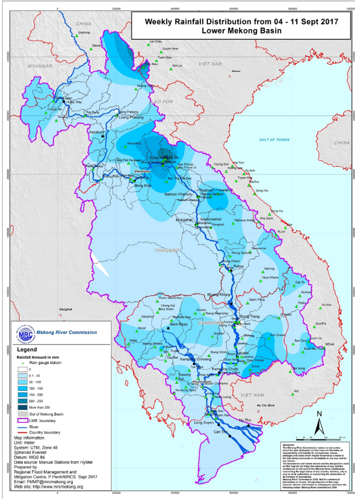
Figure 2: Weekly Rainfall Distribution over the LMB from 04 th - 11 th September 2017
