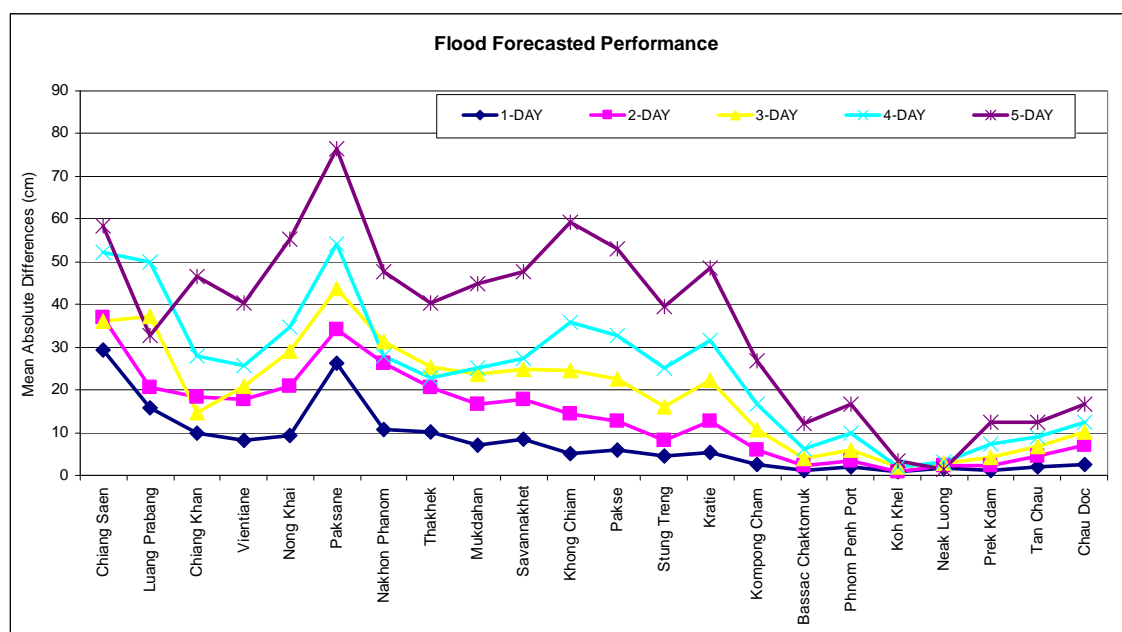
Figure B1: Average flood forecast accuracy along the Mekong mainstream (from 04 th – 11 th September 2017)
